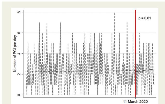
Figure 1 Time series of PCI number per day pre- and post-pandemic period with estimated slopes for the pre-pandemic period and pandemic period.
